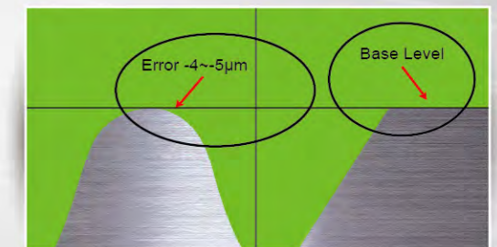
Ball-Screw (Radius Error: 4~5μm) Optical Projector Scaling: 120X
